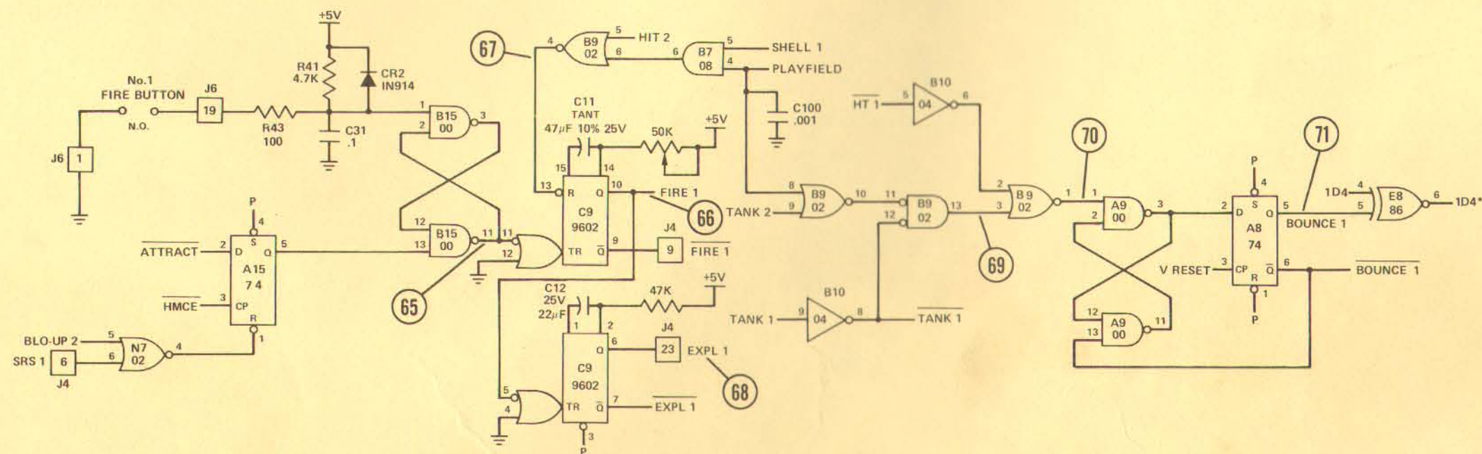
FIGURE 26 SHELL 1 CONTROL SCHEMATIC
