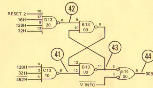
FIGURE 18 OOB SCHEMATIC
