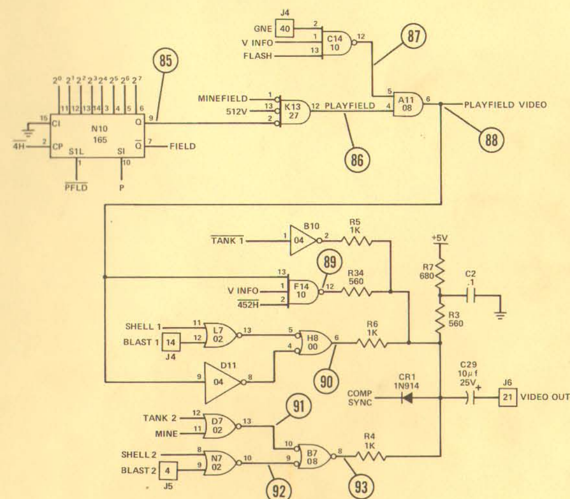
FIGURE 35 VIDEO SUMMING SCHEMATIC
