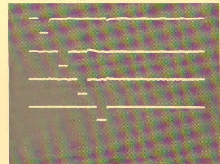
Horizontal Load Signals: This photograph illustrates the timing relationships between LDH1A, LDH1B, LDH2A, and LDH2B (top and bottom). 2 \mu s/div. 5 v/div.
