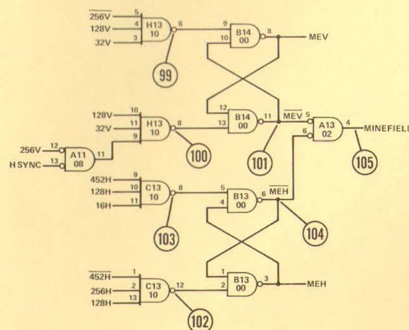
FIGURE 38 MINEFIELD SCHEMATIC
