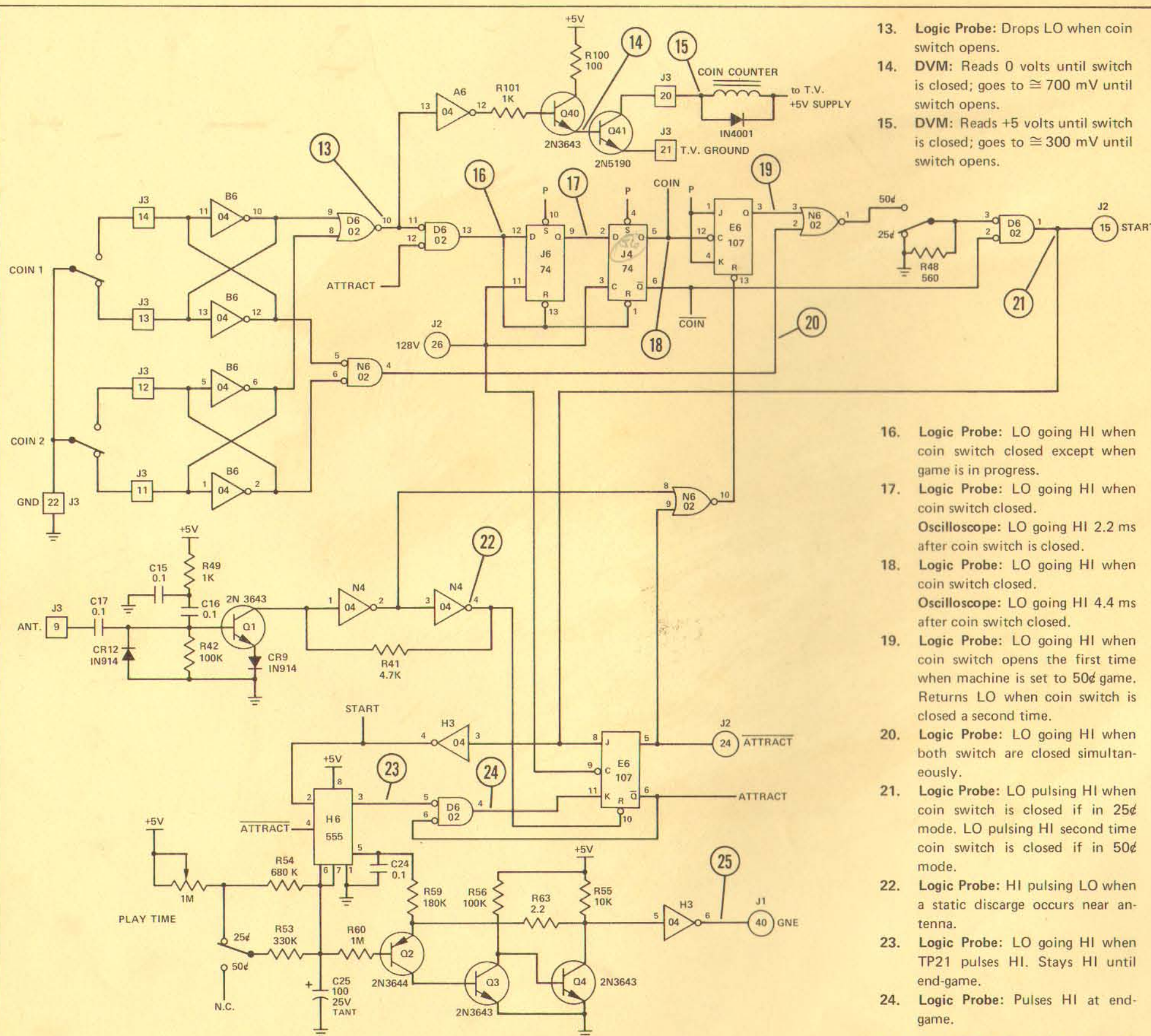
FIGURE 4 CREDIT CIRCUITRY SCHEMATIC
