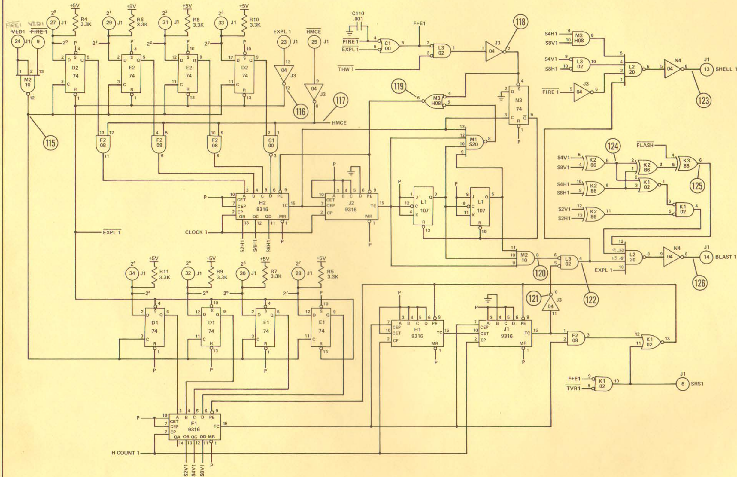
FIGURE 46 SHELL 1 MOTION CIRCUIT
