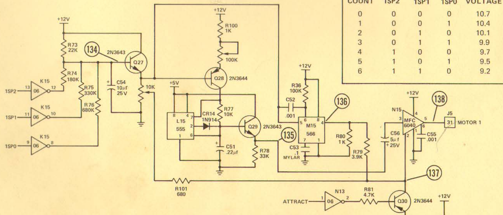
FIGURE 55 MOTOR 1 SOUND SCHEMATIC
