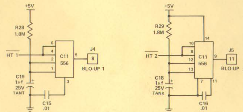
FIGURE 21 HMCE SCHEMATIC
