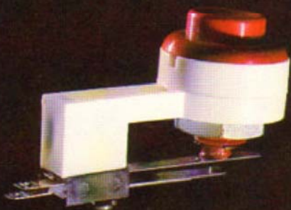
WICO PUSHBUTTON ASSEMBLY COMPLETE WITH PUSHBUTTON, HOLDER AND SWITCHES.
